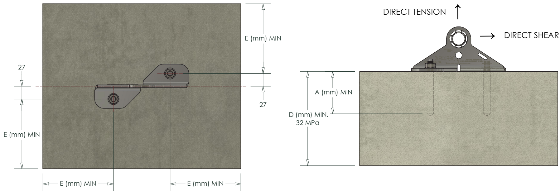
AP110 - TENSION ANCHOR CHEMICAL ANCHOR FIXING DETAILS
