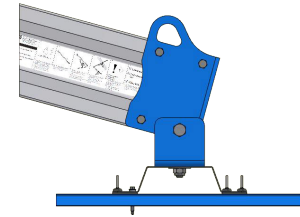
REAR ATTACHMENT - METAL ROOF MOUNT
