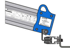
REAR ATTACHMENT - RAIL FACING HORIZONTAL DIRECTION
