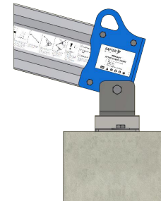
REAR ATTACHMENT - CONCRETE FLOOR MOUNT
