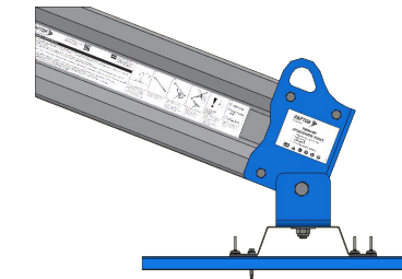
REAR ATTACHMENT - METAL ROOF MOUNT
