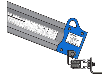
REAR ATTACHMENT - RAIL FACING HORIZONTAL DIRECTION
