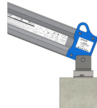
REAR ATTACHMENT - CONCRETE FLOOR MOUNT
