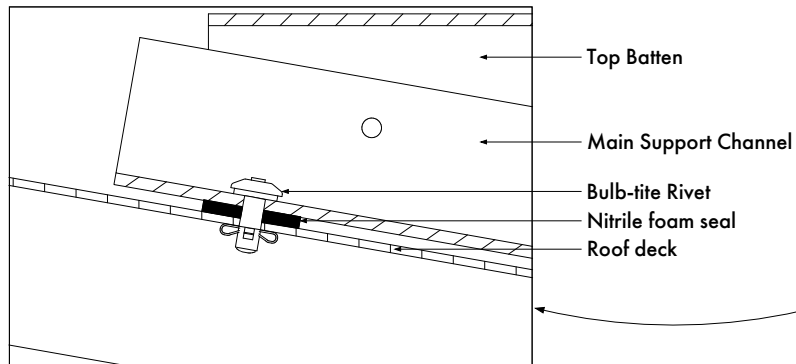
FIXING DETAILS
