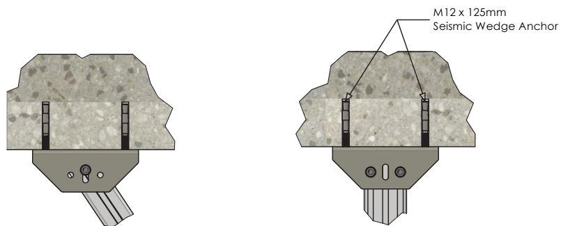
DETAIL A ( 1:10 )
