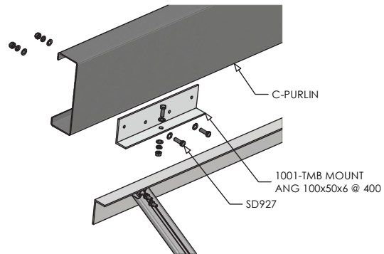
Purlin installation perpendicular to the platform
