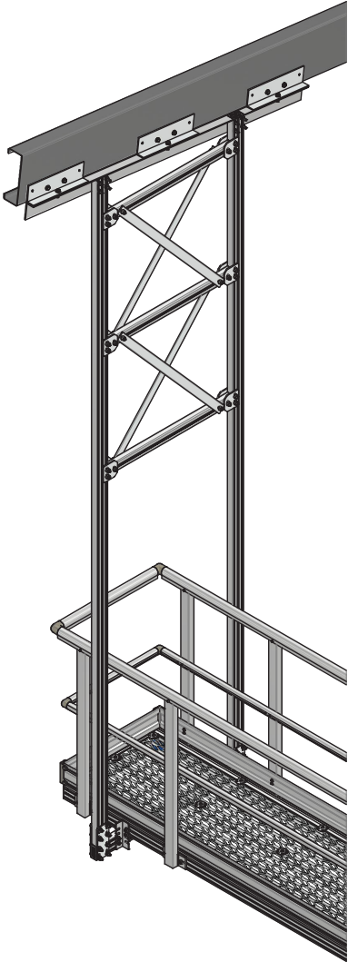
Purlin installation perpendicular to the platform
