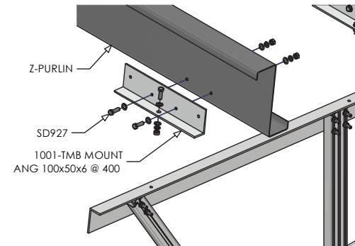
Purlin installation in-line to the platform
