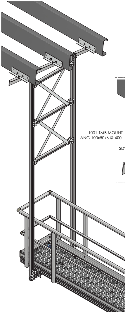
Purlin installation in-line to the platform
