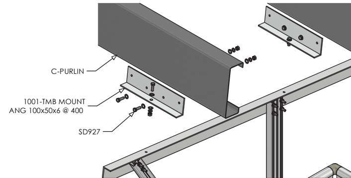
Purlin installation in-line to the platform
