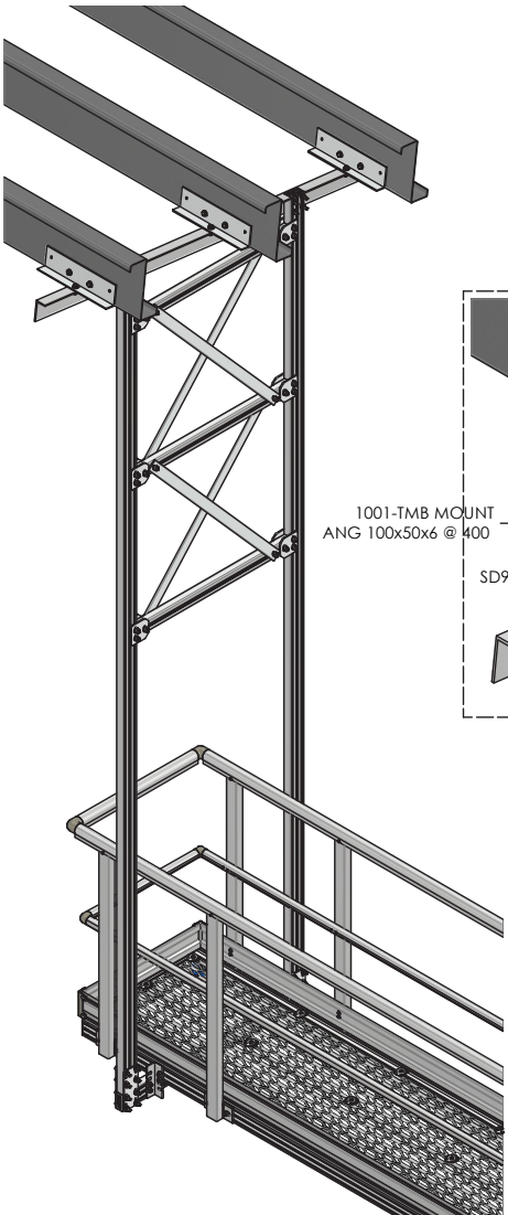
Purlin installation in-line to the platform
