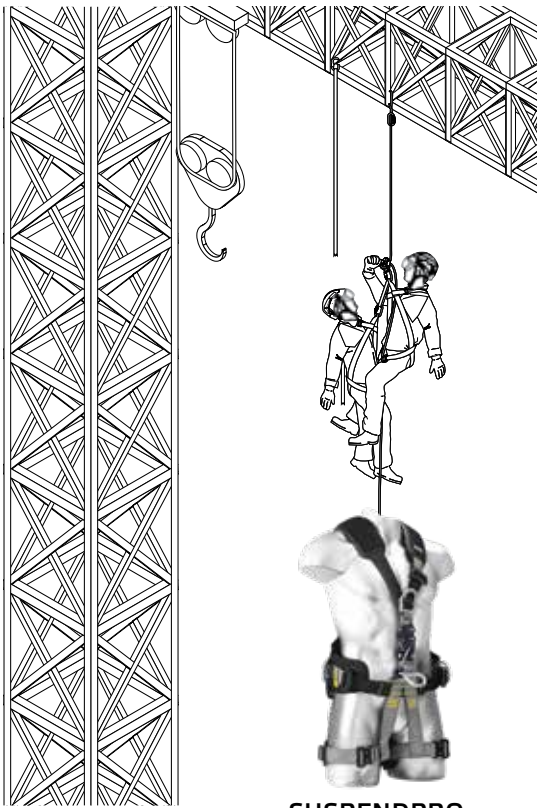
SUSPENDPRO ABSEIL HARNESS WITH INTEGRATED CHEST ASCENDER HSP4678
